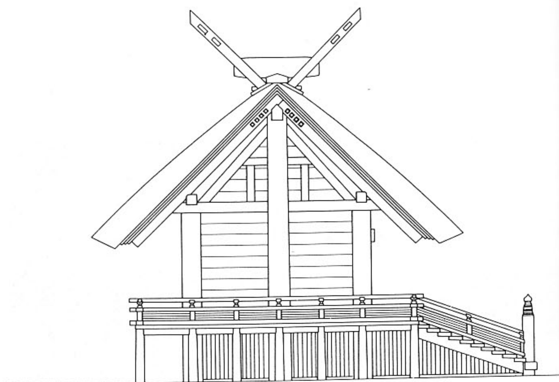
Fig 2.15 Shōden, Outer Shrine, Ise. Side elevation (1985-93 rebuilding) (Courtesy of Ise Jingū)
